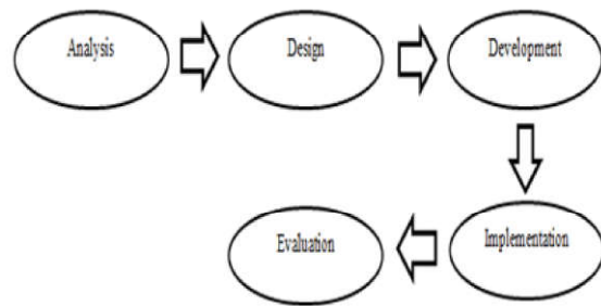
Fig.4. Model ADDIE
